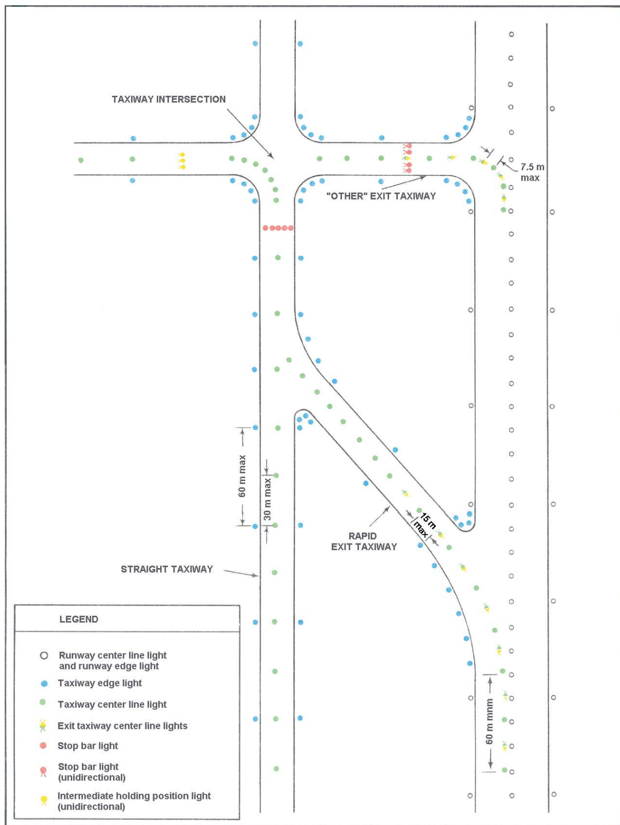
Figure 5-26. Taxiway lighting
