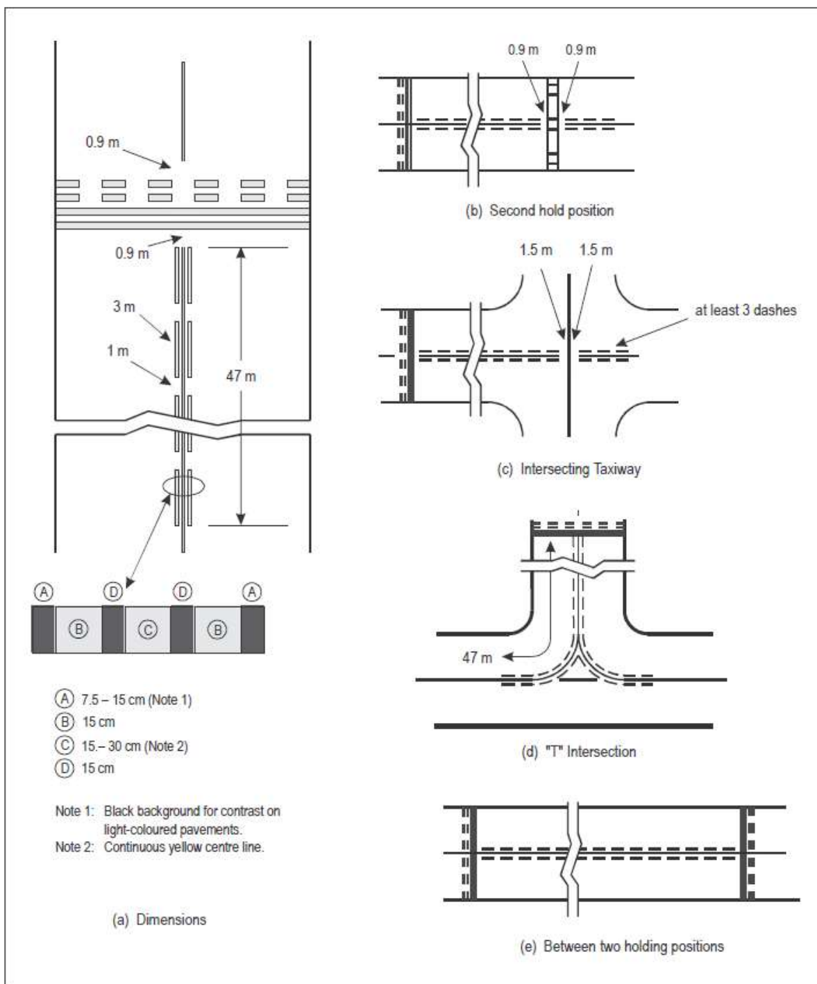
Figure 5-7. Enhanced taxiway center line marking (shown with basic runway markings)
