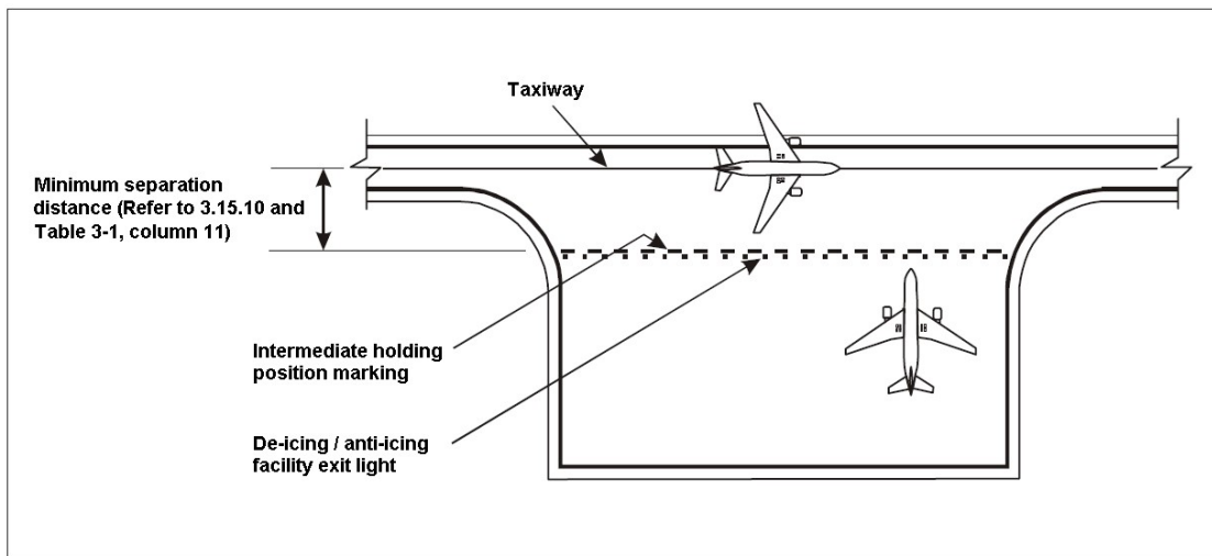
Figure 5-28. Typical remote de- icing/anti- icing facility
