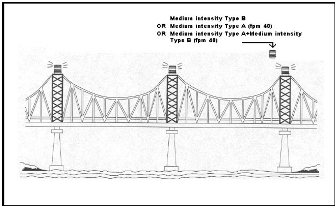
Figure 6-6. Bridge lighting
