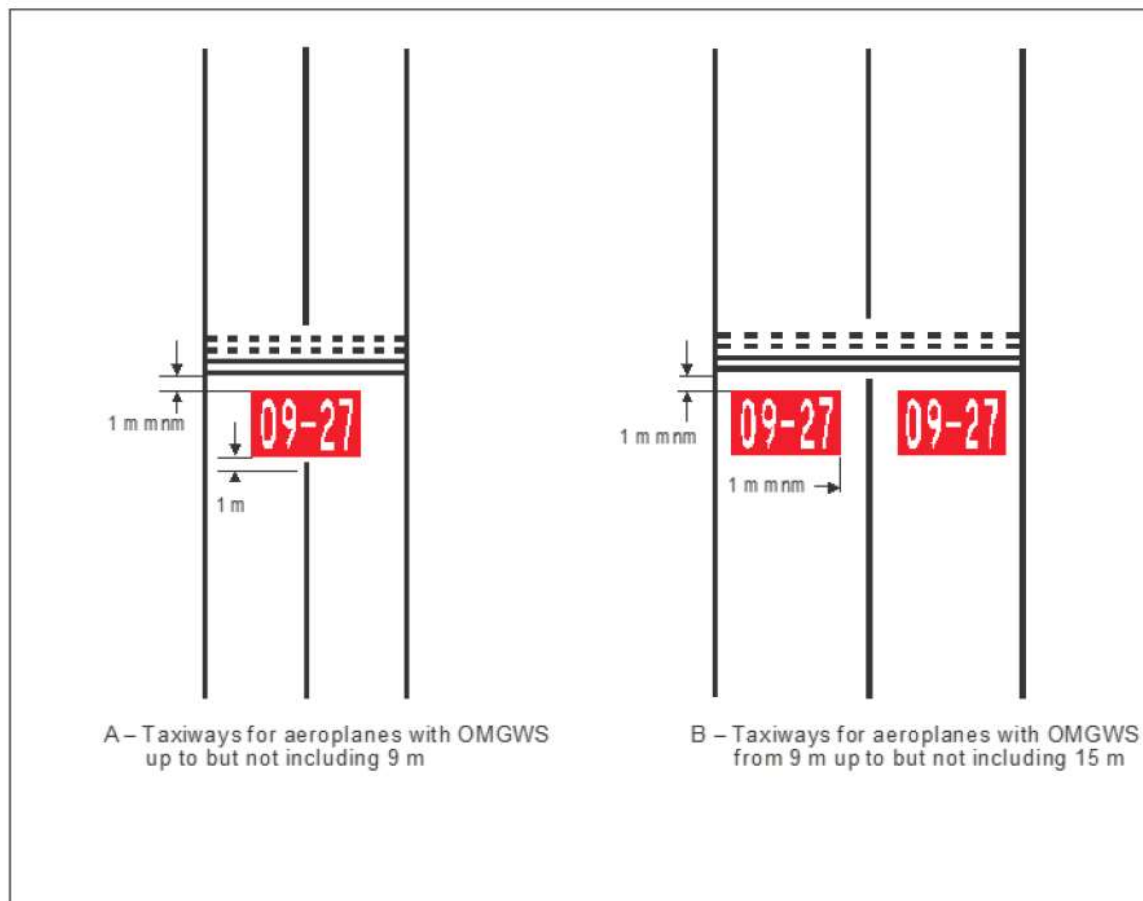
Figure 5-10. Mandatory instruction marking
