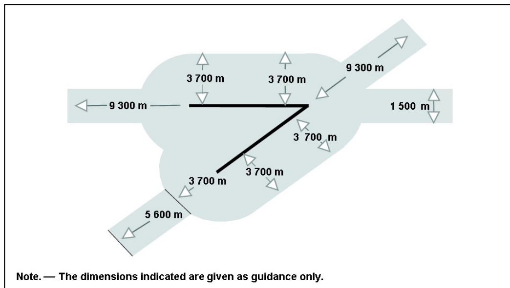
Figure 5-12. Multiple runway laser- beam free flight zone
