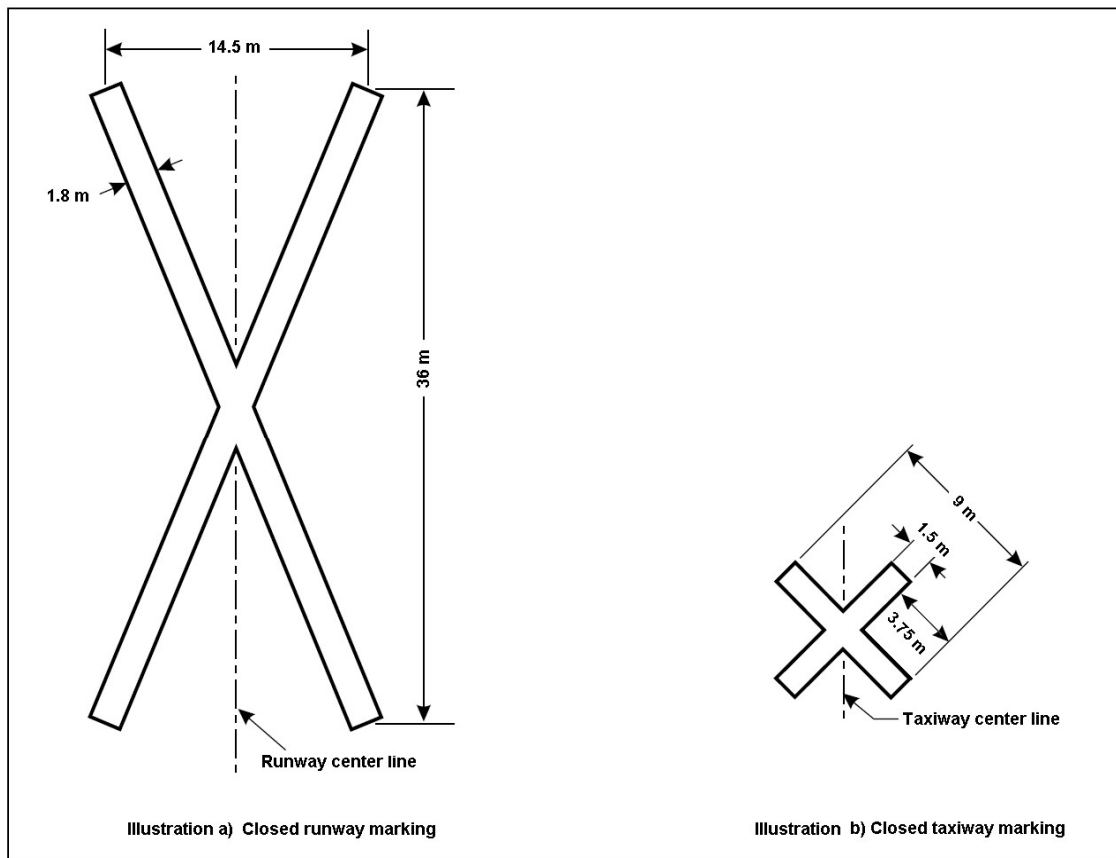
Figure 7-1. Closed runway and taxiway markings
