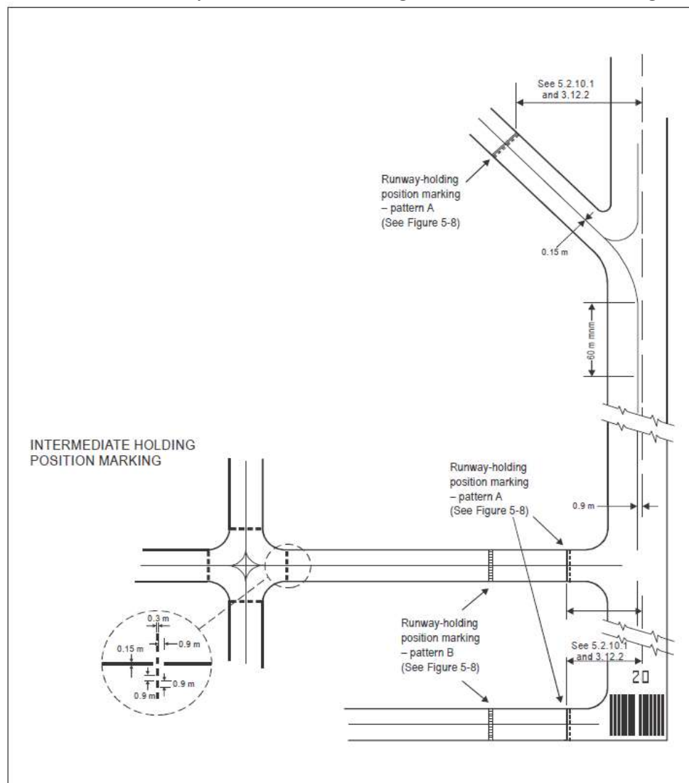
Figure 5-6. Taxiway markings (shown with basic runway markings)
