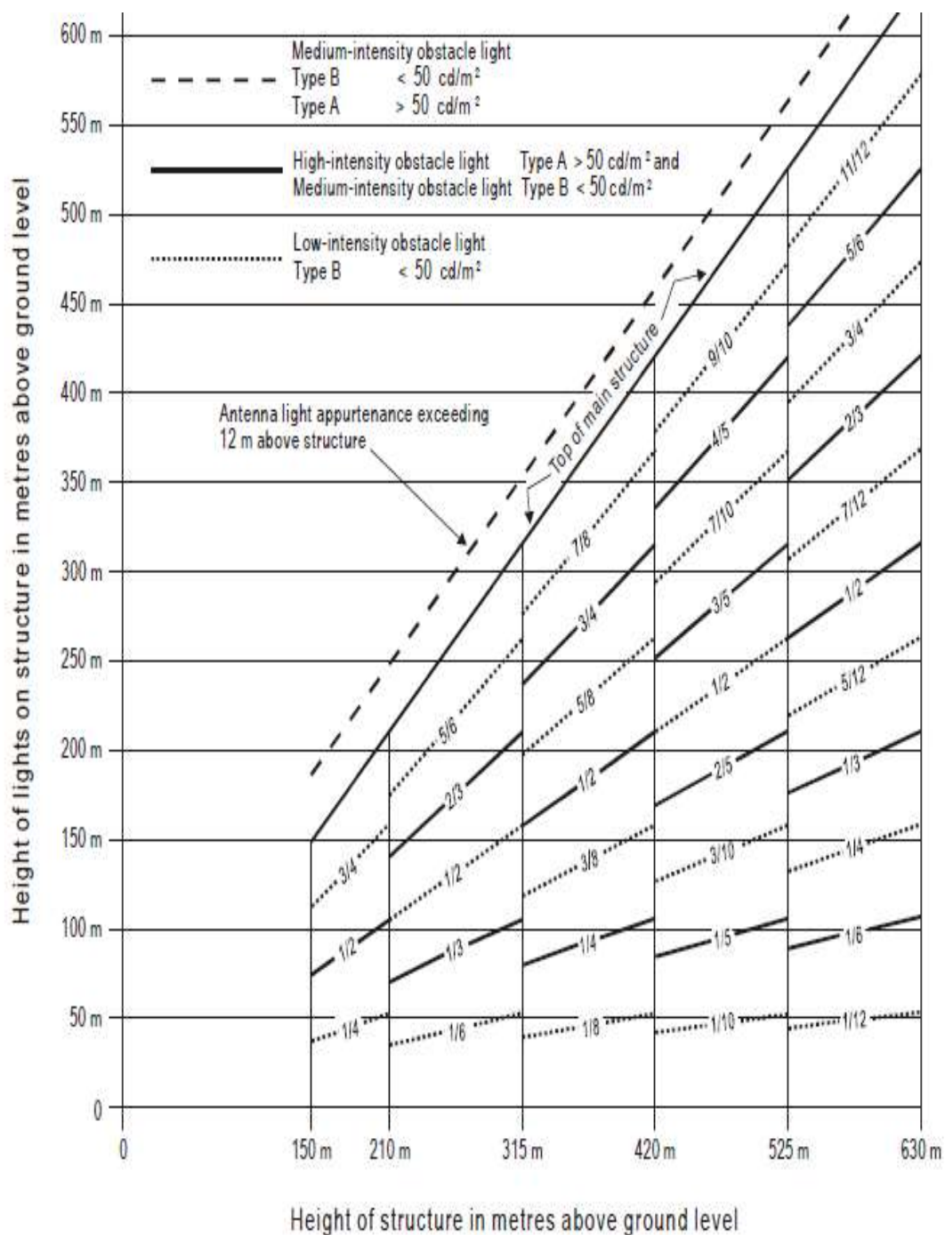
Figure 6-19. High-/medium-intensity dual obstacle lighting system, Type A/Type B
