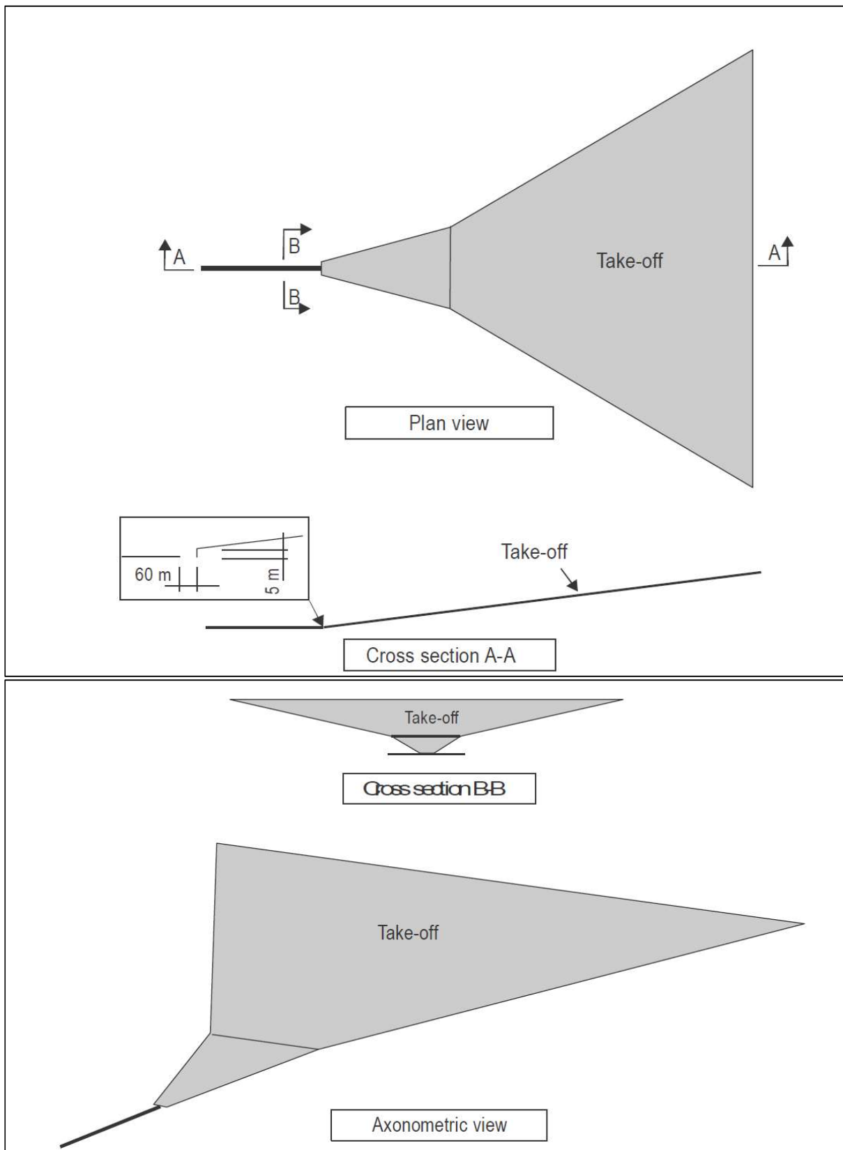
Figure 4-7. Instrument departure surface
