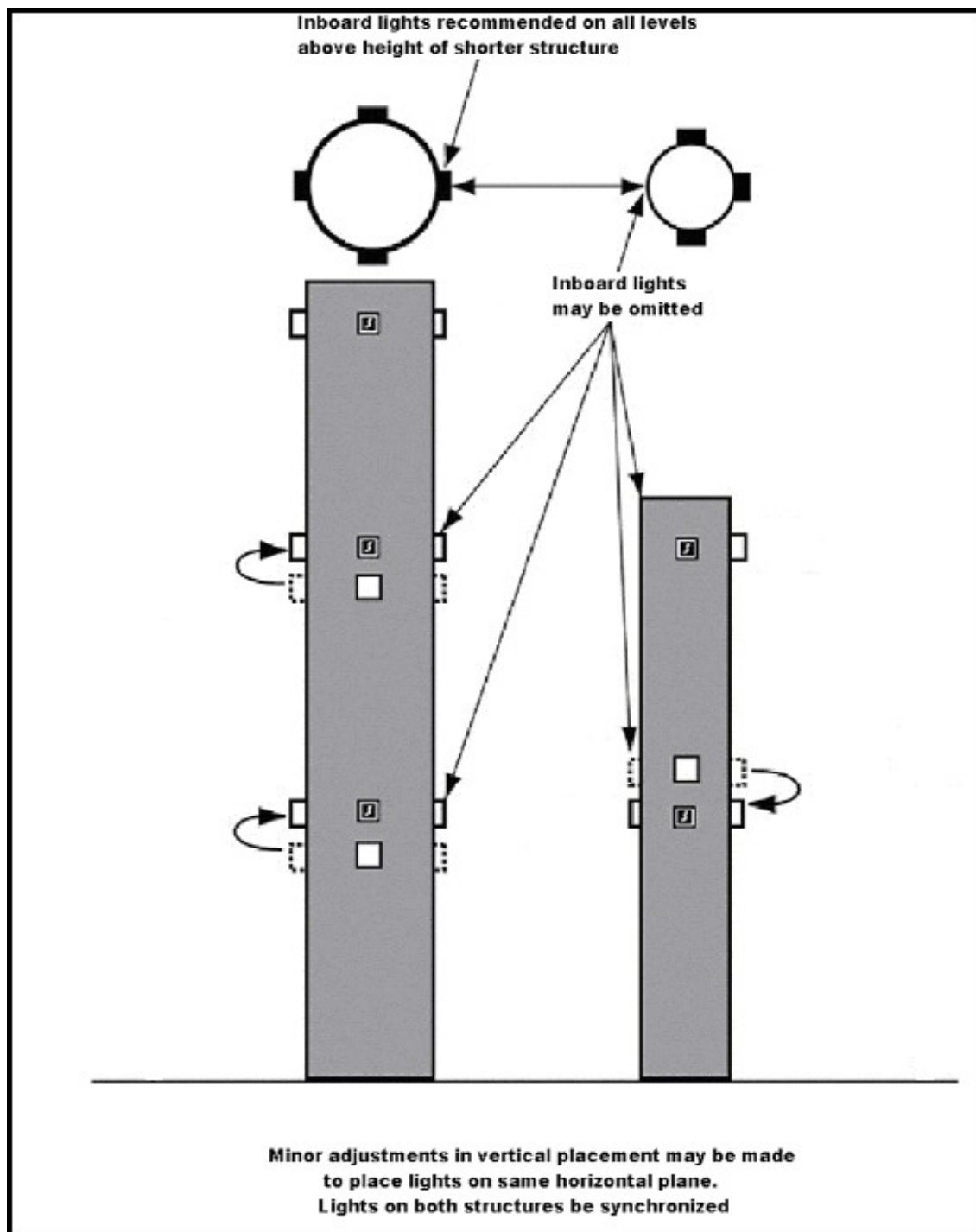
Figure 6-9. Lighting adjacent structures
