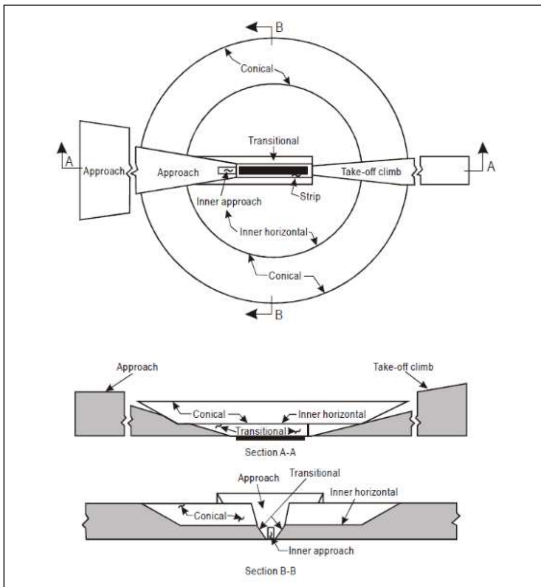
Figure 4-1. Obstacle Limitation Surfaces
