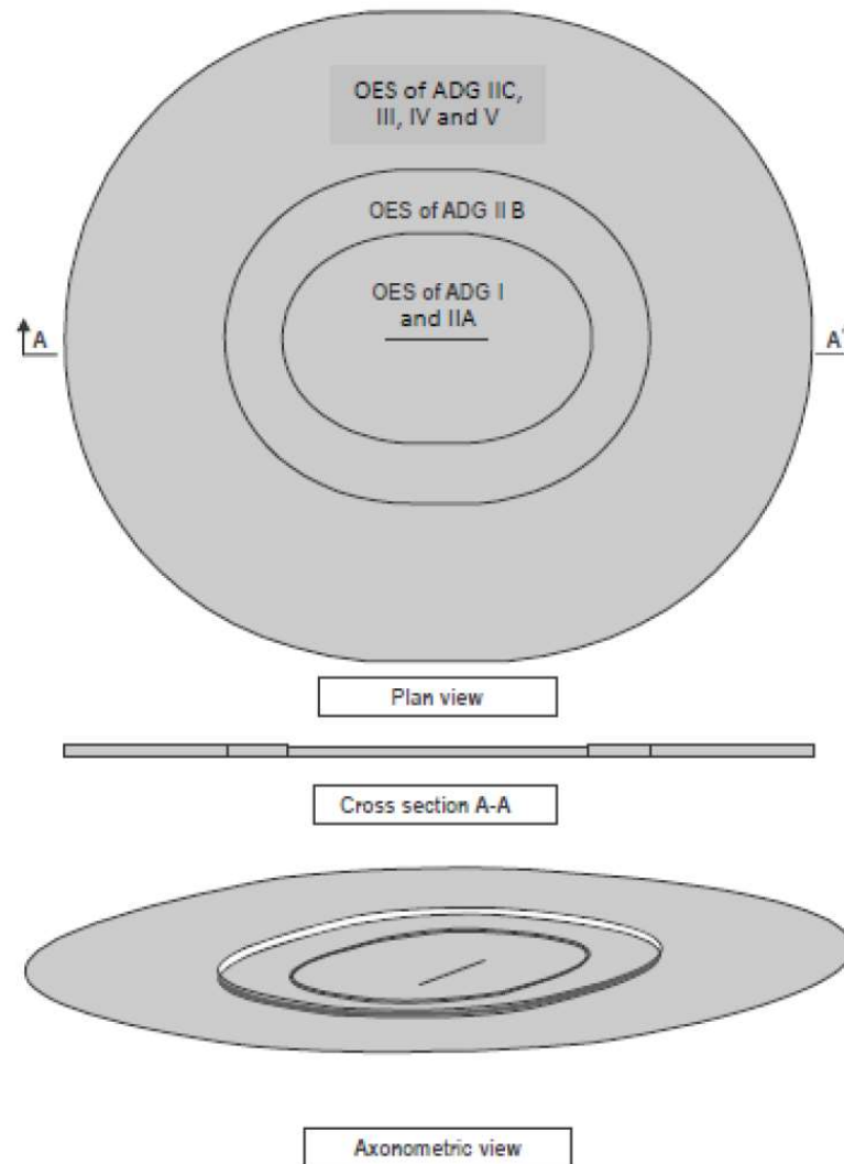
Figure 4-4. Horizontal surface
