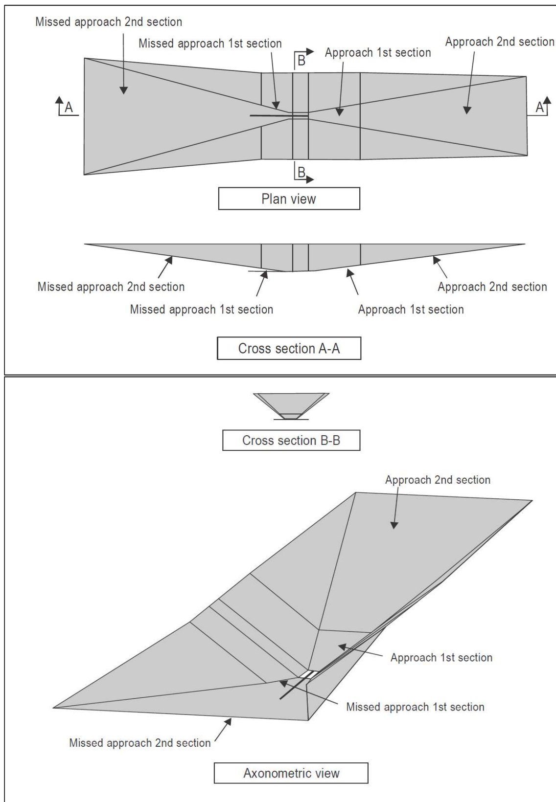
Figure 4-6. Surface for precision approaches
