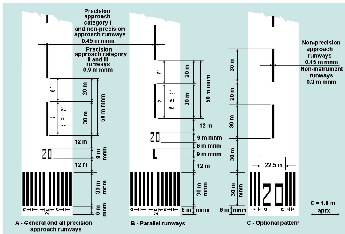
Figure 5-2. Runway designation, center line and threshold markings
