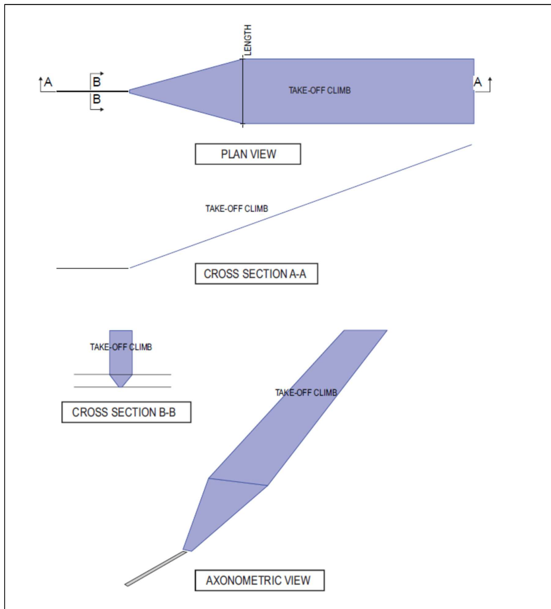
Figure 4-8 Take-off climb surface
