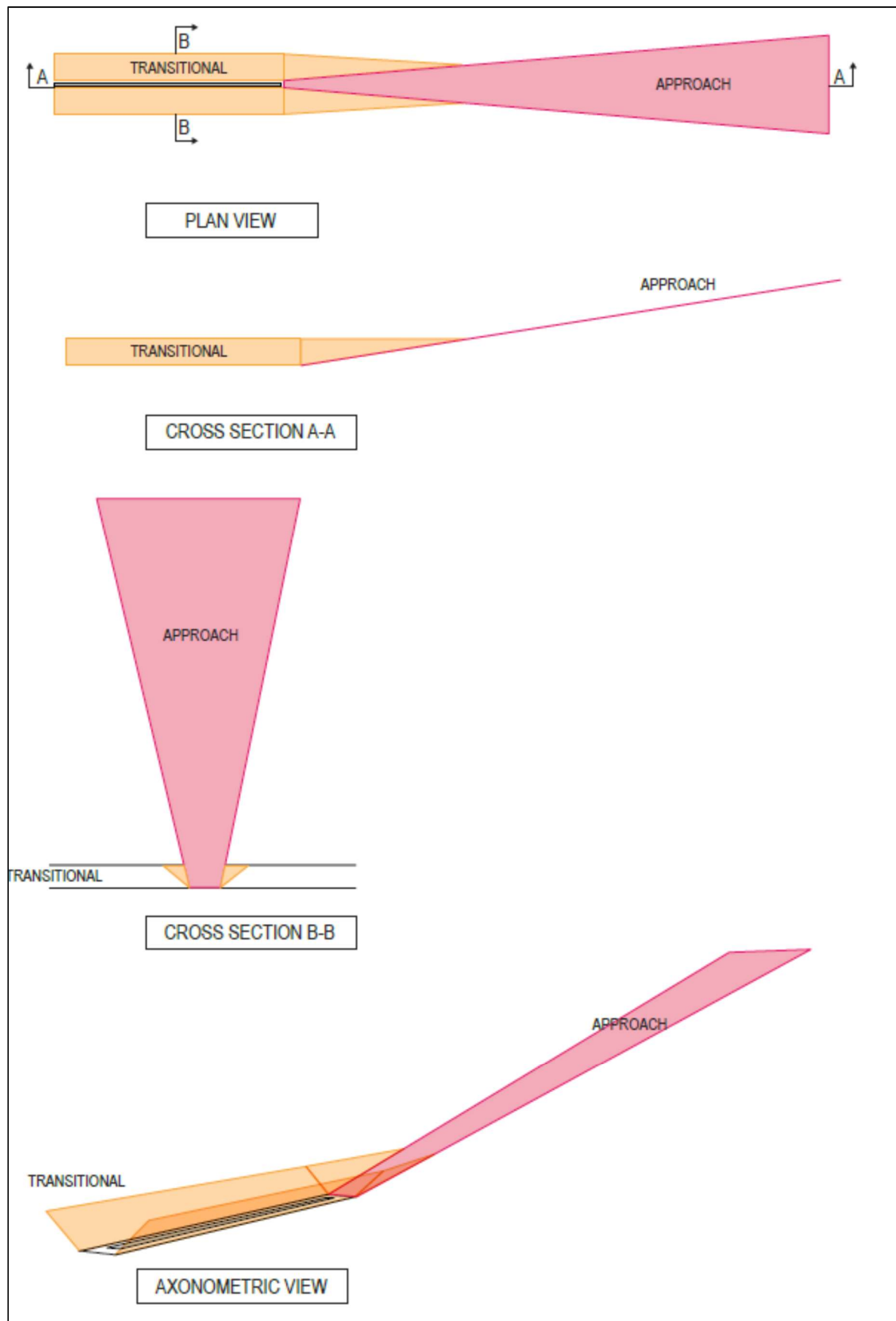
Figure 4-1. Approach surface and transitional surfaces
