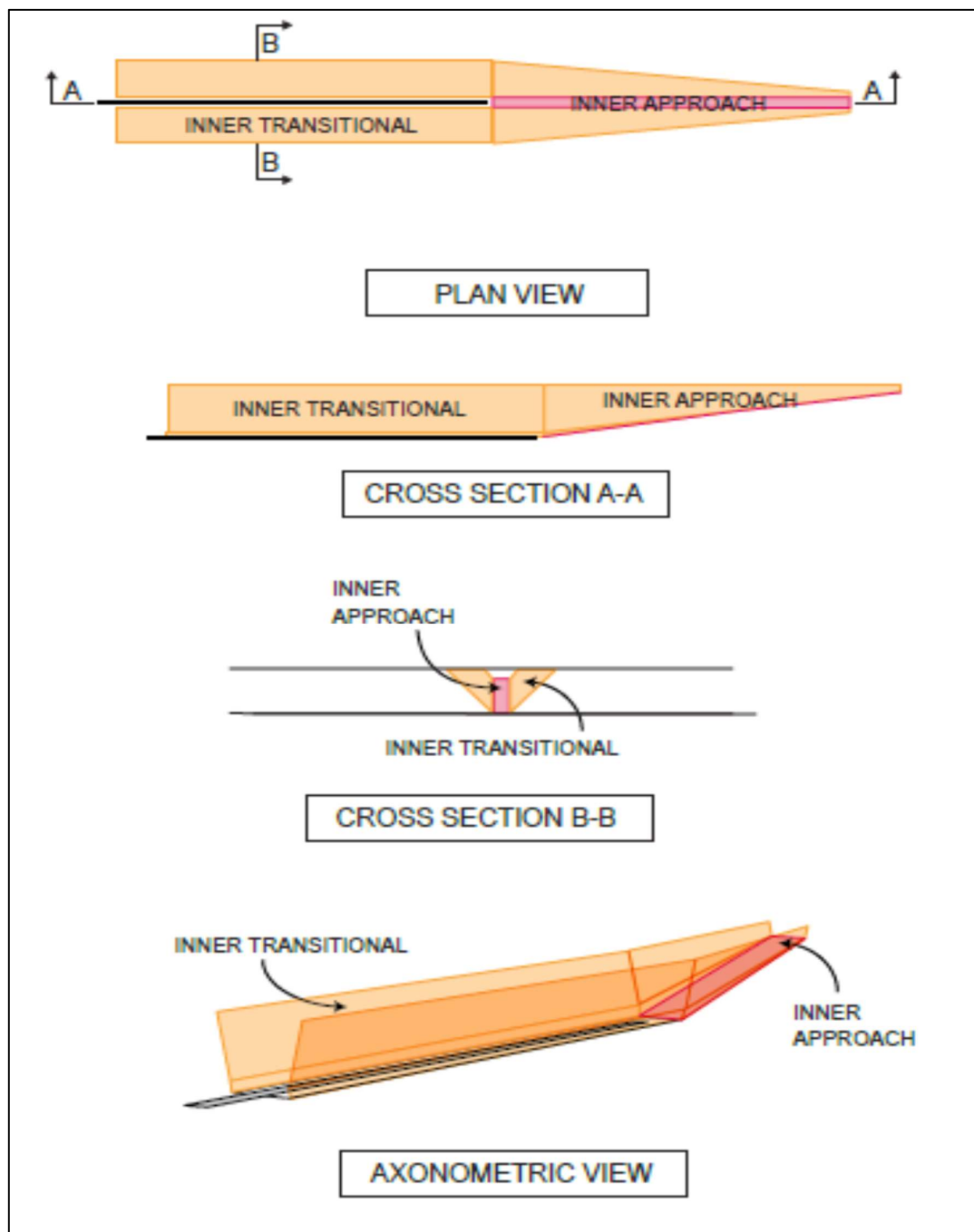
Figure 4-2. Inner approach and inner transitional surfaces on a non-precision approach runway
