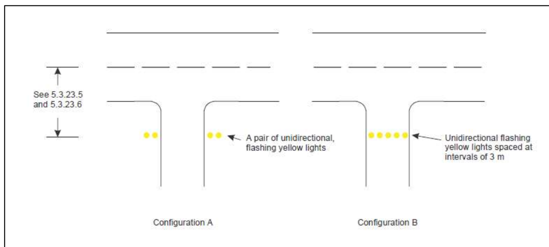
Figure 5-29. Runway guard lights
