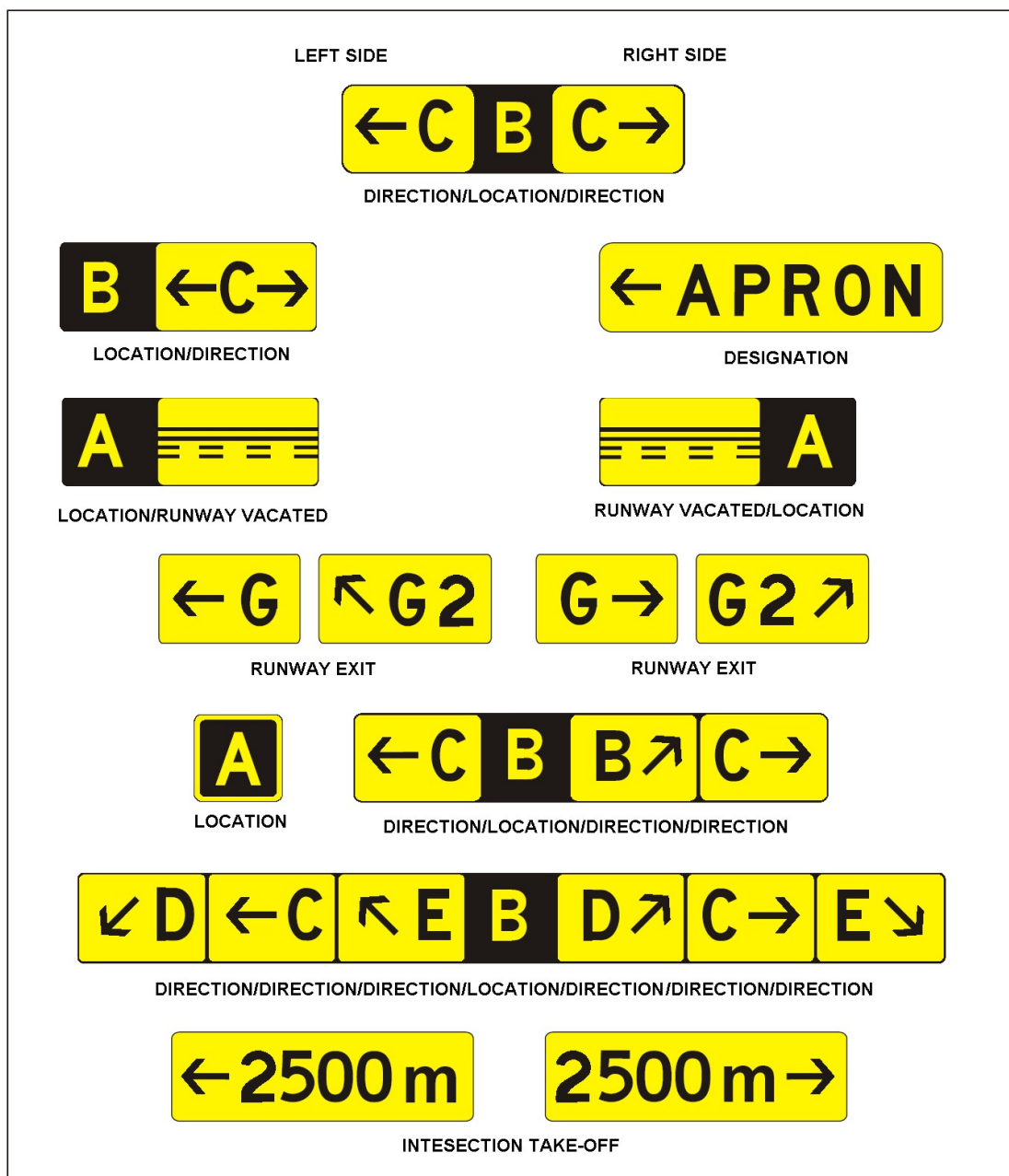
Figure 5-31. Information signs
