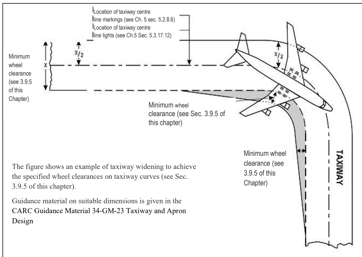
Figure 3-2. Taxiway curve
