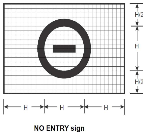
Figure A4-3. Runway vacated and NO ENTRY signs
